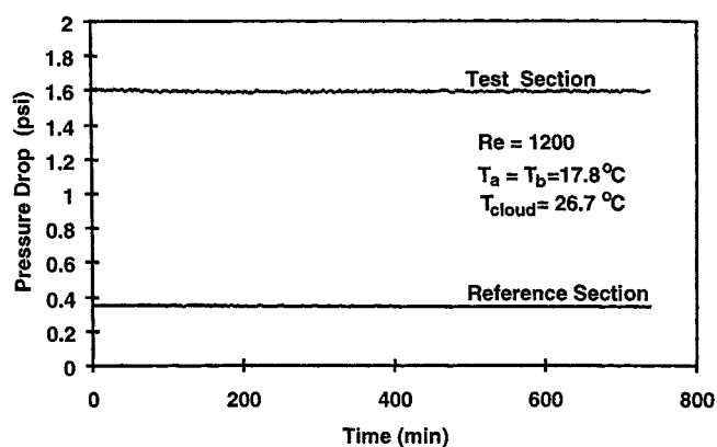
Figure 12. Pressure drop in the reference and test section during the flow of the oil below the cloud point at a Reynolds number of 1,200.
