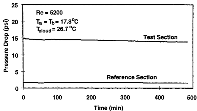
Figure 13. Pressure drop in the reference and test section during the flow of the oil below the cloud point at an average Reynolds number of 5,200.
